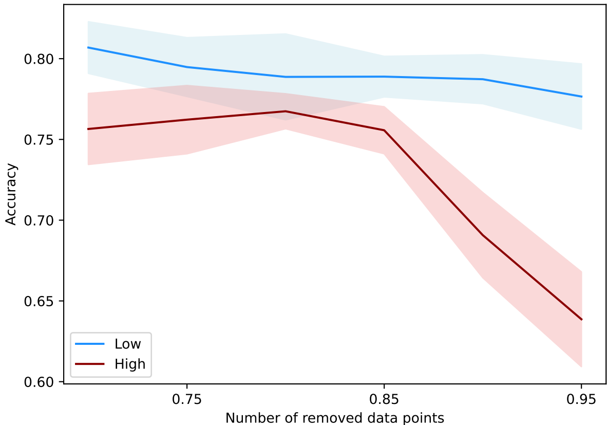
DataAttrOpt(5000, 0.03, 15, max+s, alpha=best) - imdb-embeddings
